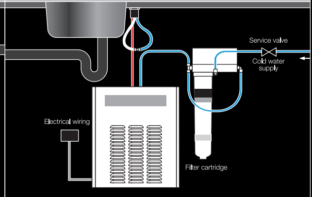
Zip Chill Tap Under Sink Installation
