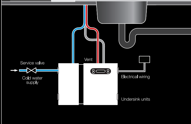
Zip HydroTap Under Sink Installation
